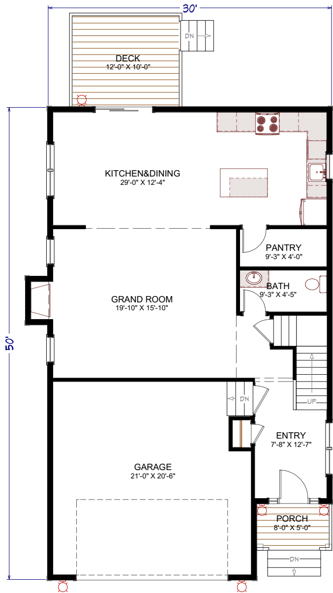
1st Floor LIVING AREA 979 SQ FT
