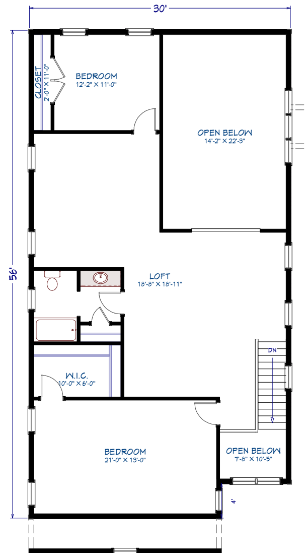
2nd Floor
