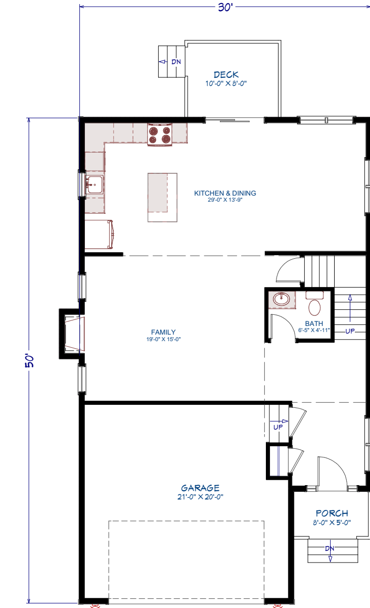
1st Floor
