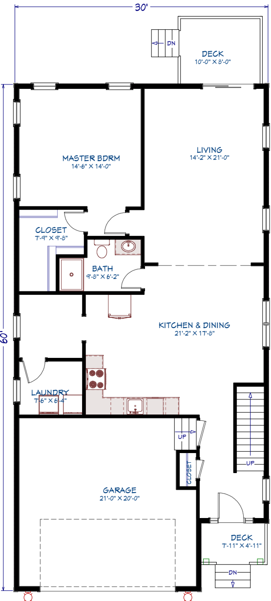
1st Floor LIVING AREA 1301 SQ FT
