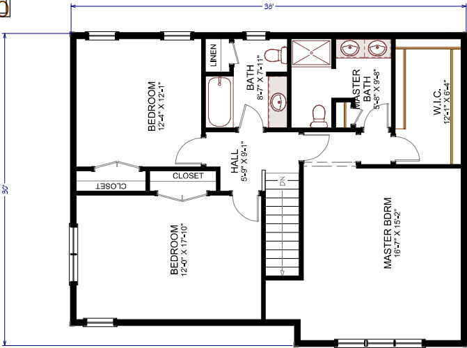
2nd Floor LIVING AREA 1097 SQ FT
