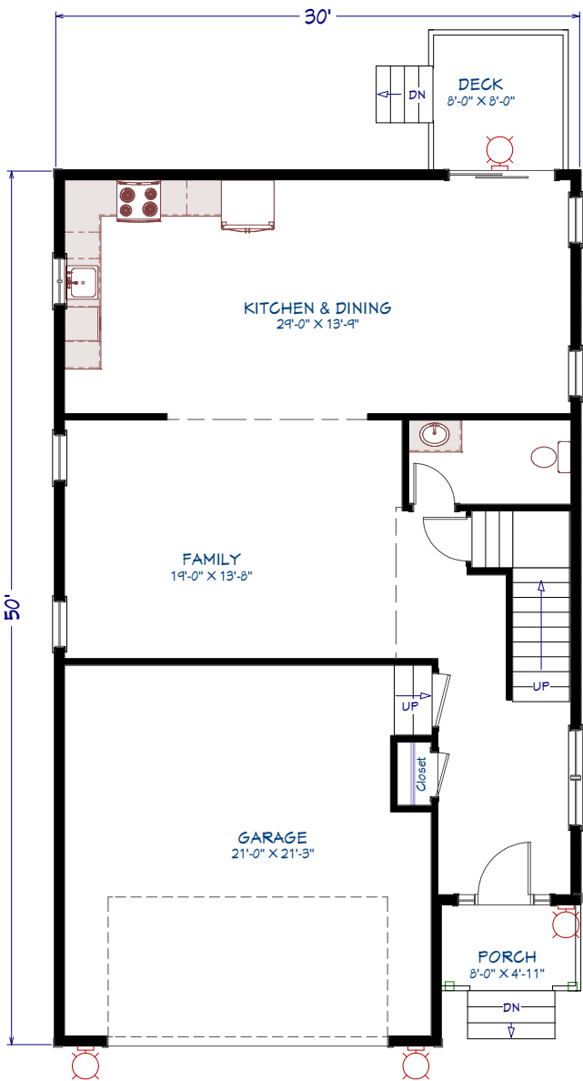
1st Floor LIVING AREA 972 SQ FT
