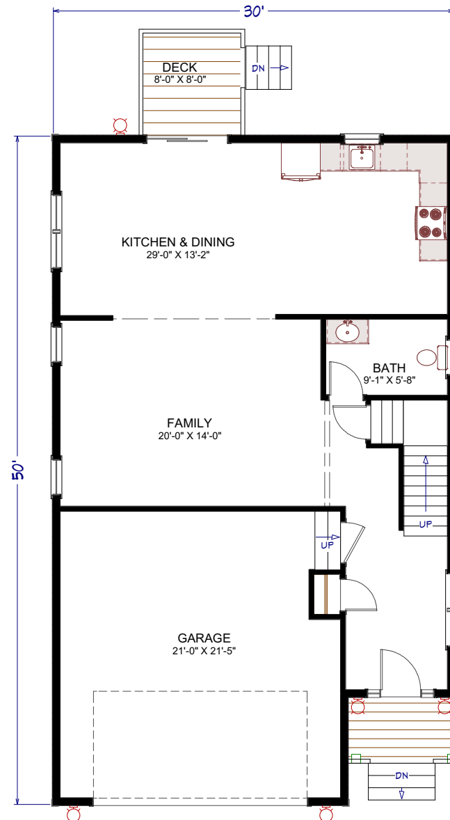
1st Floor
