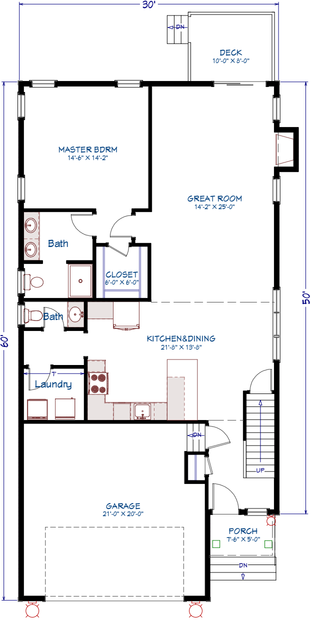
1st Floor LIVING AREA 1274 SQ FT
