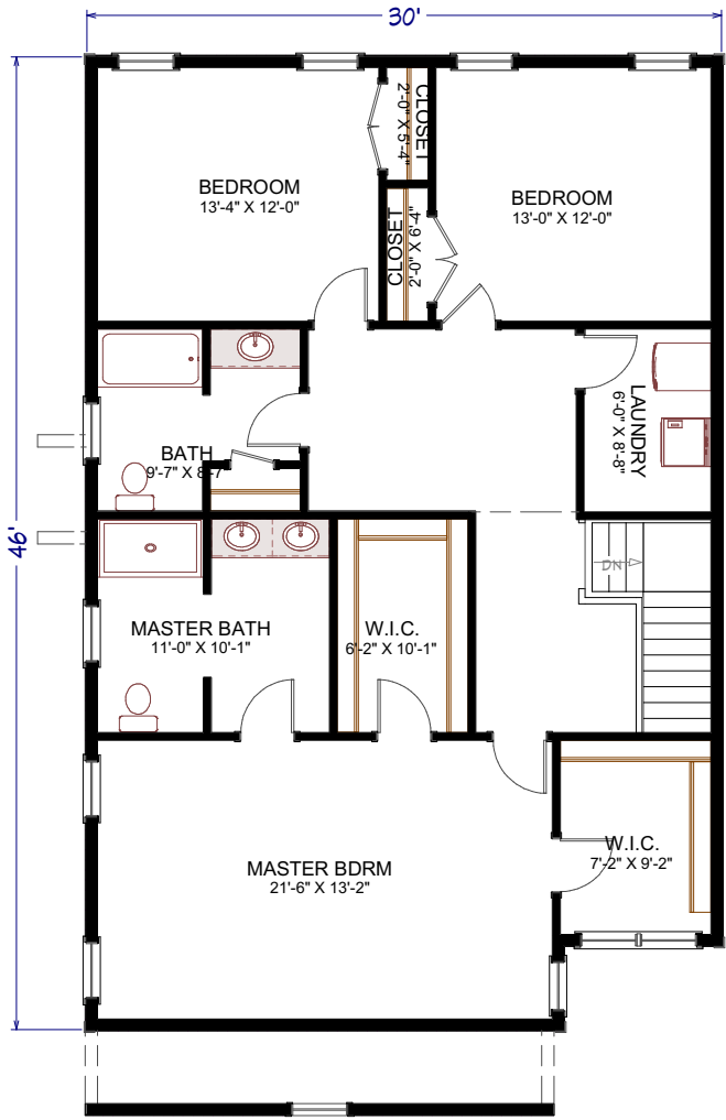
2nd Floor LIVING AREA 1302 SQ FT
