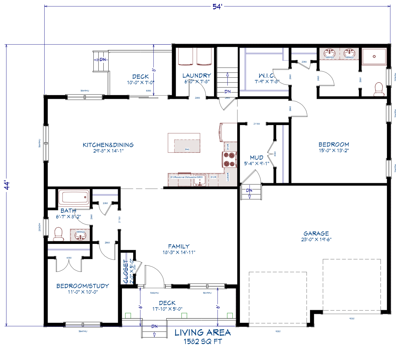
1st Floor
