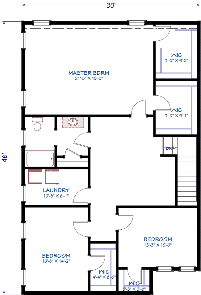
2nd Floor LIVING AREA 1295 SQ FT
