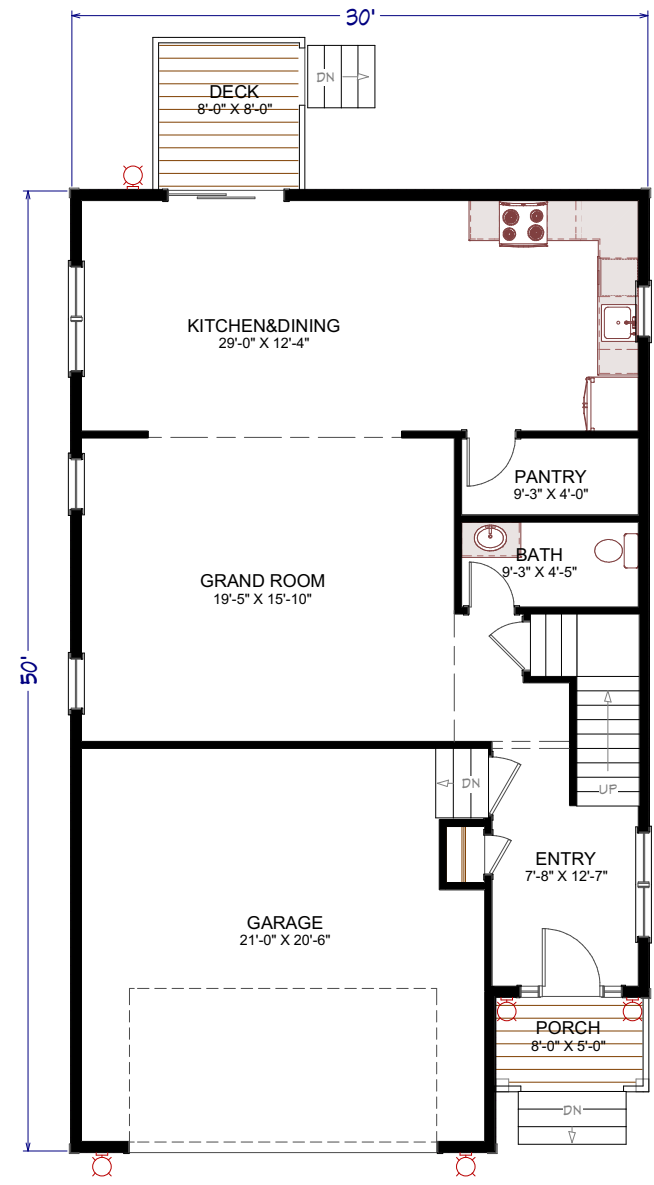
1st Floor
