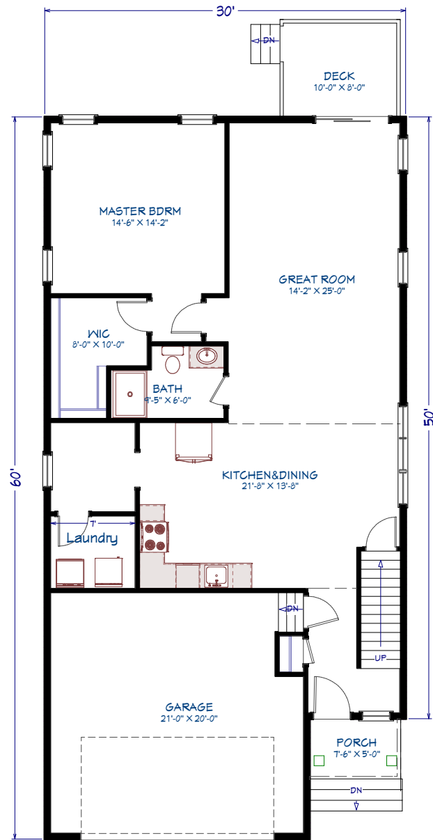
1st Floor
