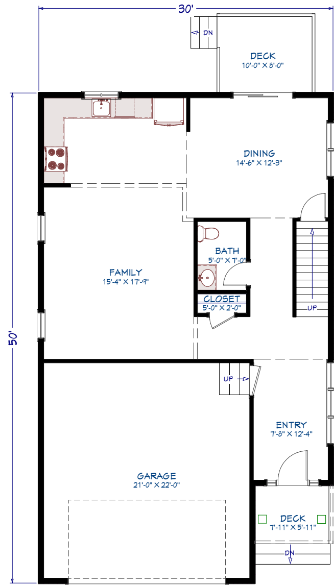
1st Floor LIVING AREA 931 SQ FT
