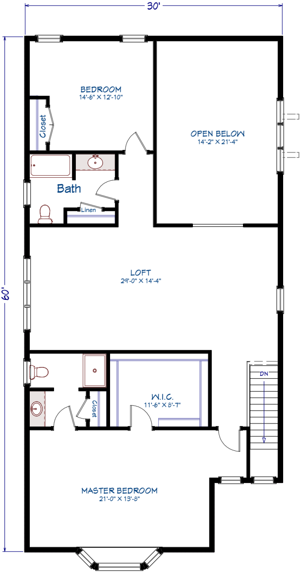
2nd Floor
