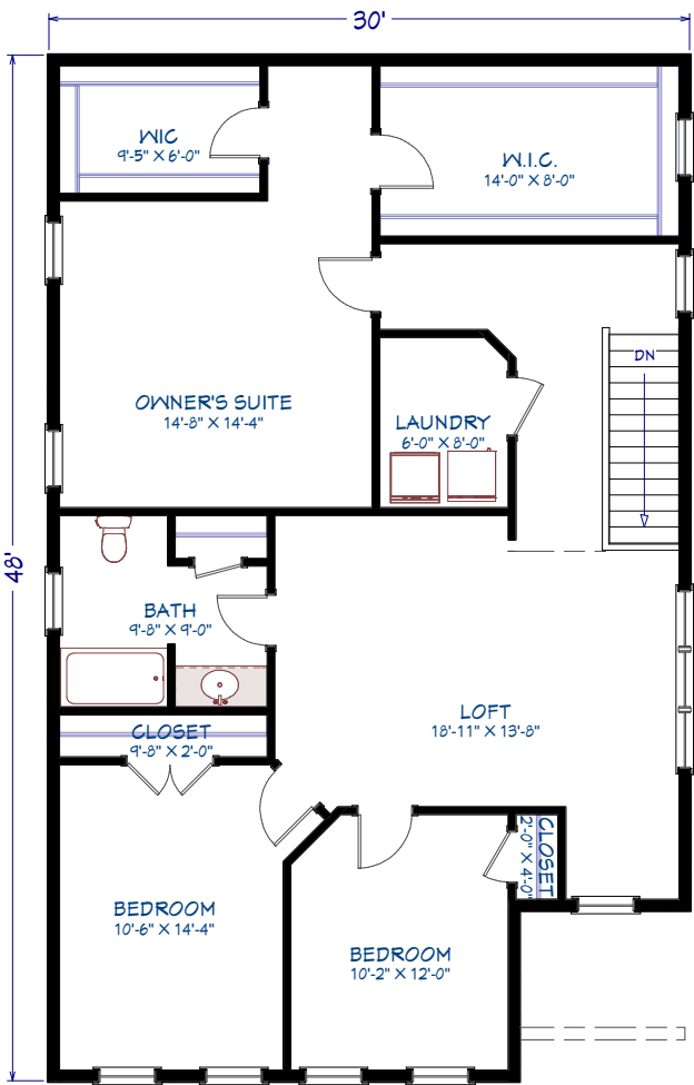
2nd Floor LIVING AREA 1339 SQ FT
